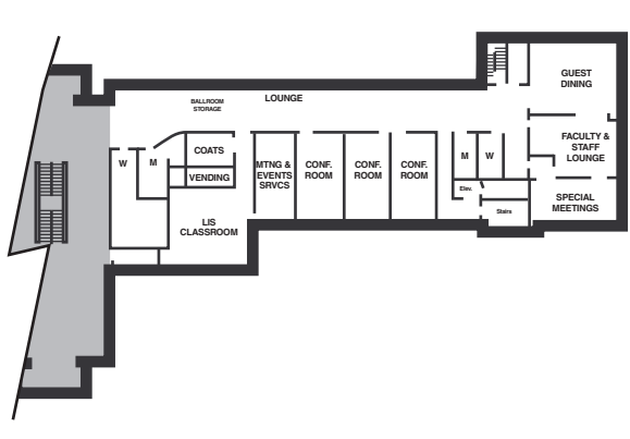
Coeur de Catherine — 3rd Floor
